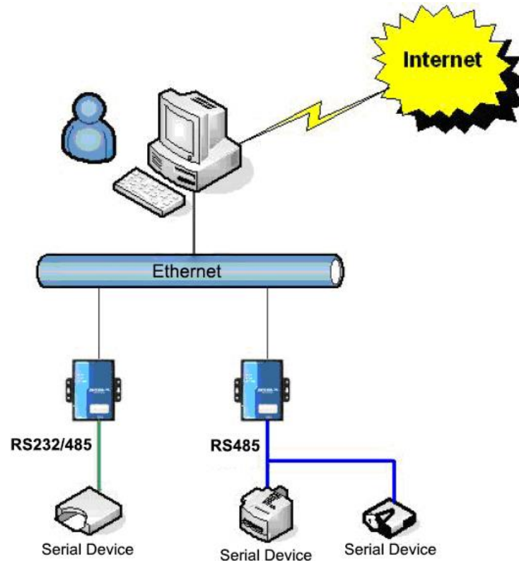
Figure 2 ITT-SR-1RS1FE-WiFi Network Structure
