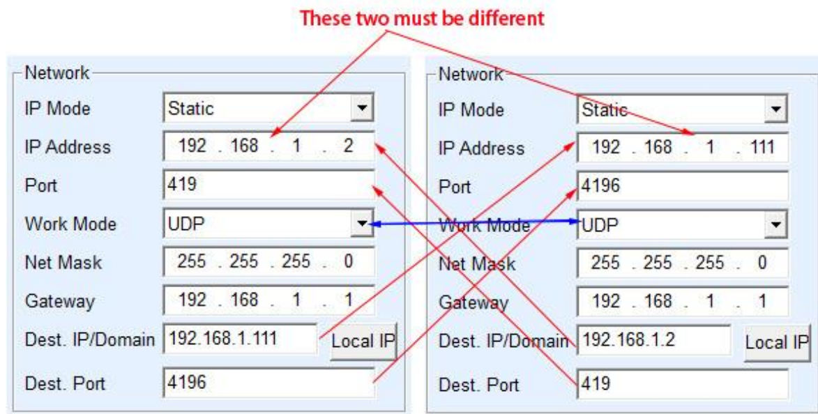
Figure 33 UDP Device Pair-connection Configuration
