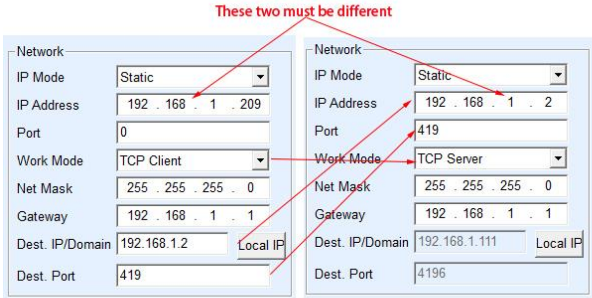
Figure 31 TCP Device Pair-connection Configuration
