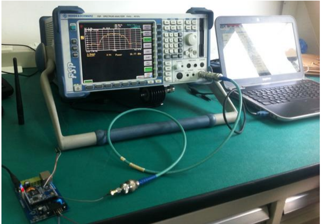
Figure 10 ITT-SR-1RS1FE-WiFi Signal Test
