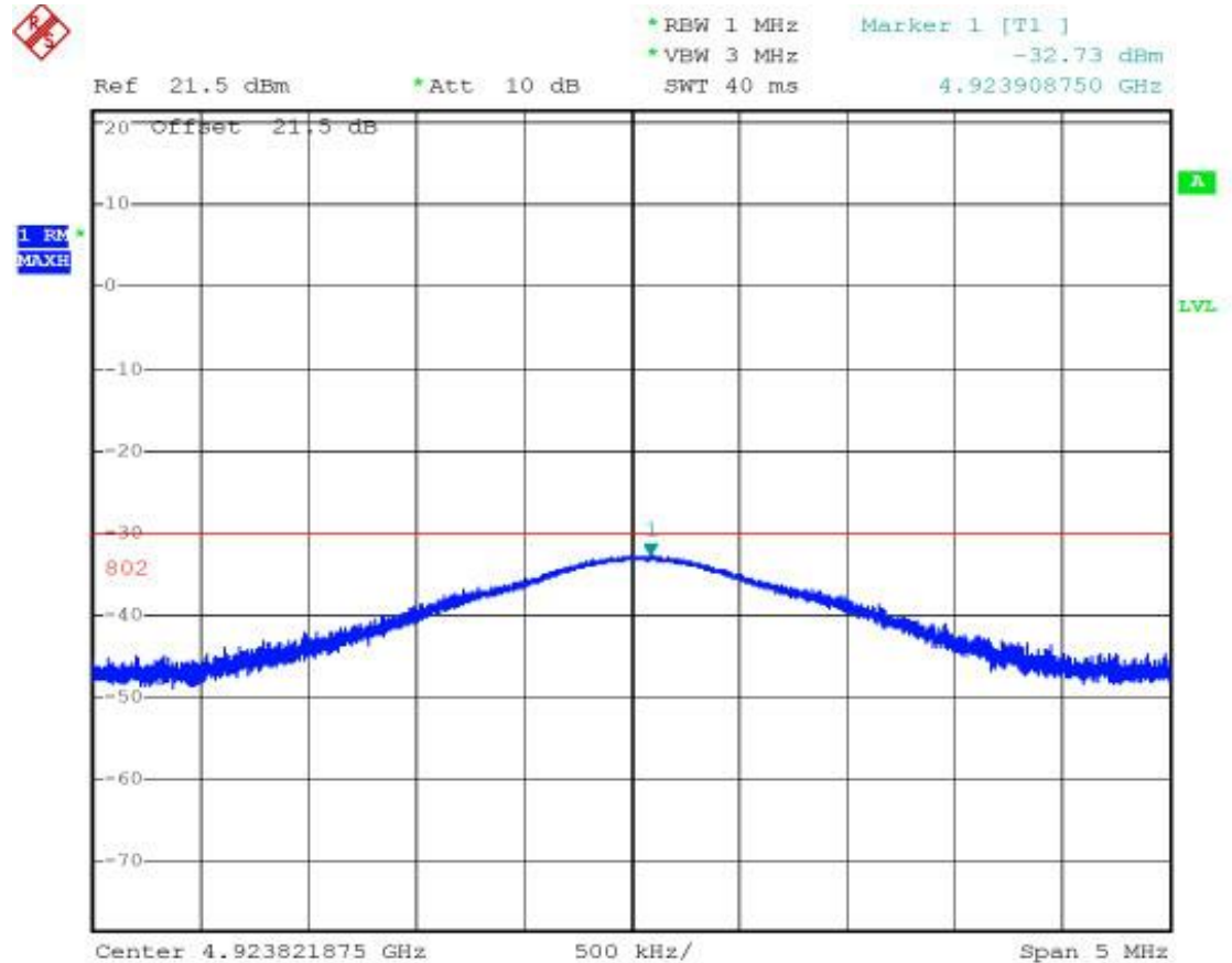
Figure 13 ITT-SR-1RS1FE-WiFi Stray Test Curve
