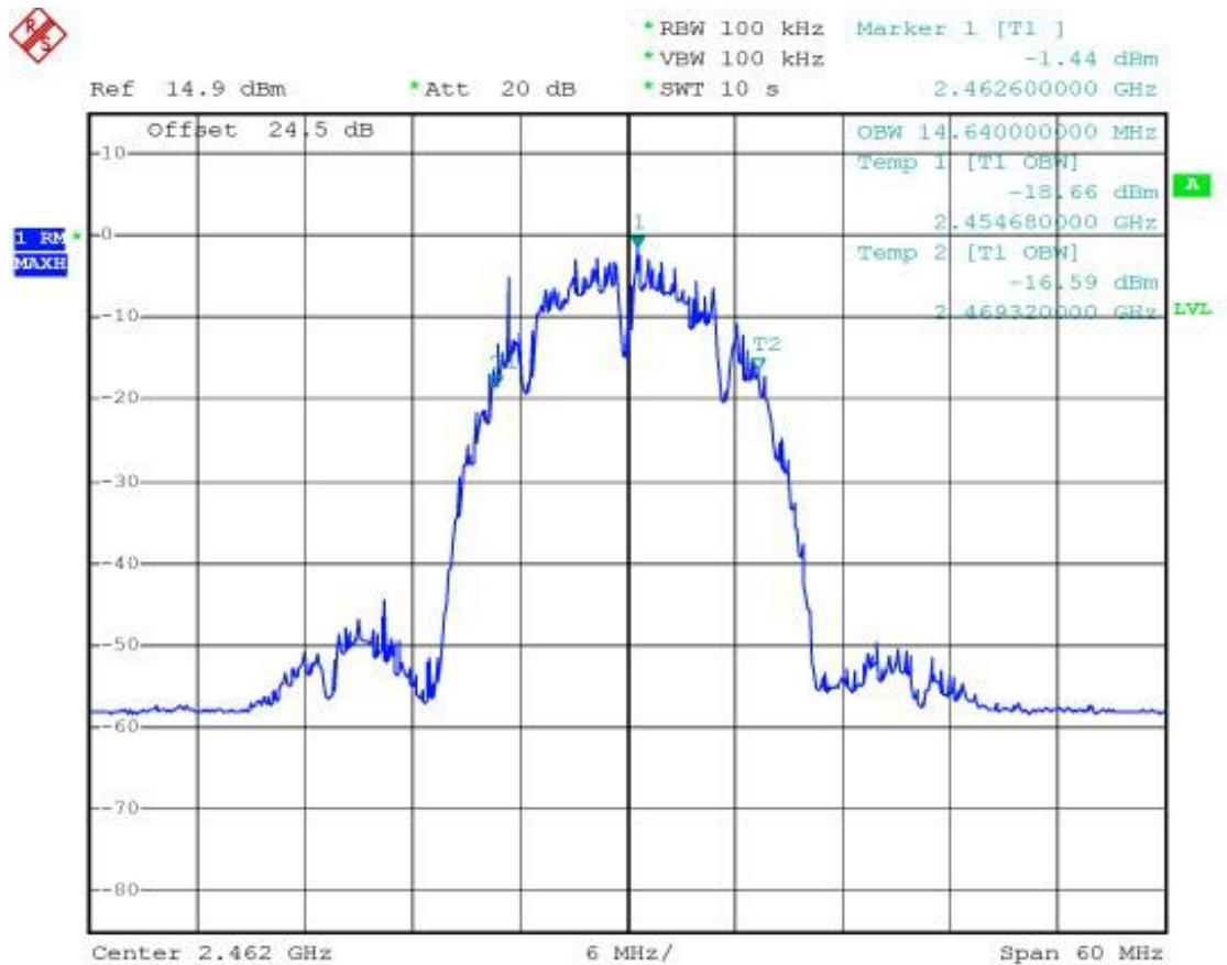
Figure 11 ITT-SR-1RS1FE-WiFi Bandwidth Test Curve
