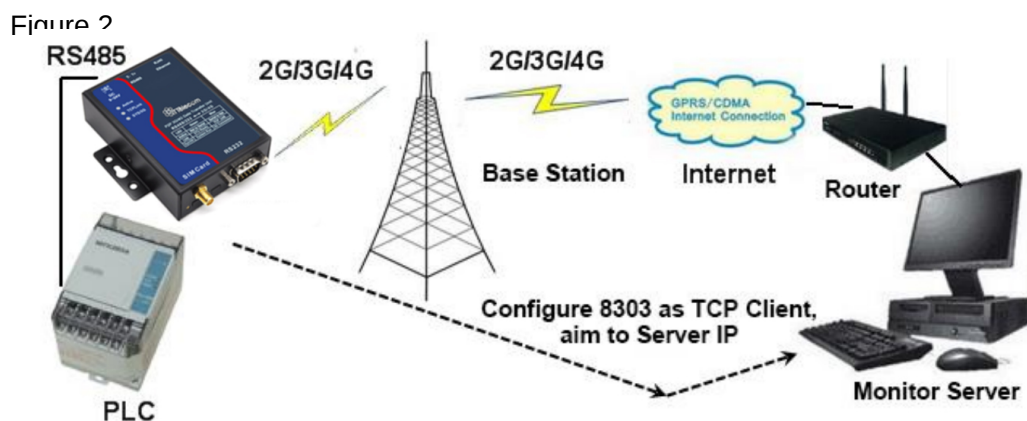
Figure 2 Normal 3G/4G DTU Mode
